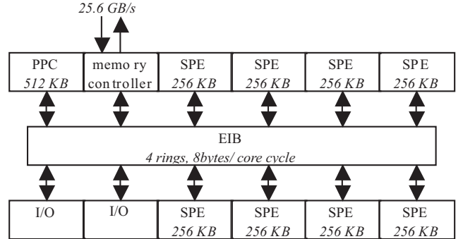
Figure 1: Overview of the Cell processor
