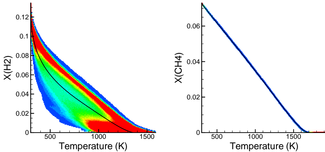
Figure 7. Joint PDF of temperature and H_2 . For comparison, we present a comparable joint PDF for a methane flame. In both cases, the black line represents fuel versus temperature for a corresponding flat laminar flame.
