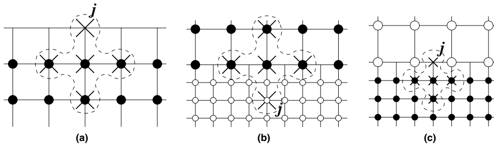
Fig. 2. Cases in which data at non-valid nodes is needed in computing the discrete Laplacian at a valid node. Nodes of the stencil are indicated by \times , valid nodes at the current level by \bullet . (a) Stencil reaches physical boundary (at top point). (b) Stencil is partially covered by the next finer level (at bottom point). (c) Stencil intersects boundary with coarser level (at top point).
