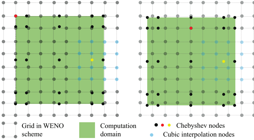
Fig. 4.1: The computation of f(\mathbf{r}_i^c, \mathbf{r}_j^c) in a 2D domain (shown as the green area) with f = \tau^2, v_0, v_1 . Here r_i^c, i = 1, \dots, N_I denote the Chebyshev nodes with N_I = 5^2 (the black dots). Two instances of \mathbf{r}_j^c are shown: for each instance, a fast sweeping method with a grid size h_0 , grid points \mathbf{r}_i^0 and a point source collocated at one Chebyshev node (the red dot) is used to compute f(\mathbf{r}_i^0, \mathbf{r}_j^c) . For each \mathbf{r}_i^c, i \neq j (the yellow dots), f(\mathbf{r}_i^c, \mathbf{r}_j^c) is computed via cubic interpolation from the grid points \mathbf{r}_i^0 (the blue dots).
