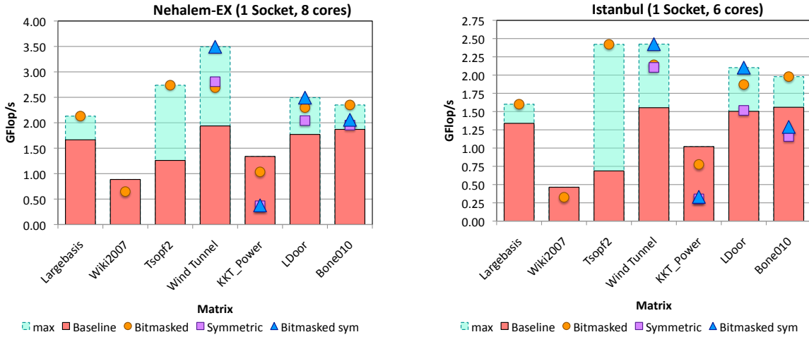
Fig. 12: Parallel performance of SpMV kernels on Nehalem-EX (left) and Istanbul (right). Baseline original CSB code is in red; circles show bitmasked register blocks; triangles and squares show symmetric algorithm with and without bitmasked register blocking, respectively; green shows overall performance gain of our approach. The first three matrices are unsymmetric, followed by four symmetric matrices. The unsymmetric algorithms (‘Baseline’ and ‘Bitmasked’) run on original matrices while the symmetric algorithms (‘Symmetric’ and ‘Bitmasked sym’) run on RCM ordered matrices.
