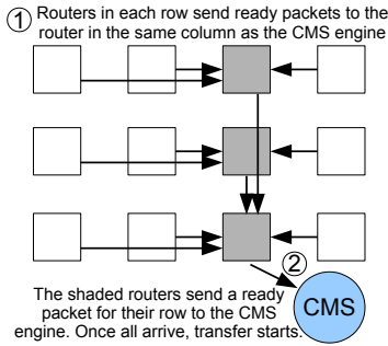
Figure 3: Initiating a synchronous read CMS operation.
