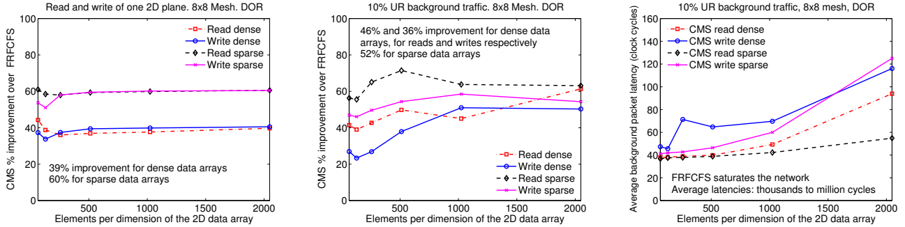
Figure 10: CMS transfer completion time improvement over FRFCFS (uncoordinated) and the impact on background traffic.
