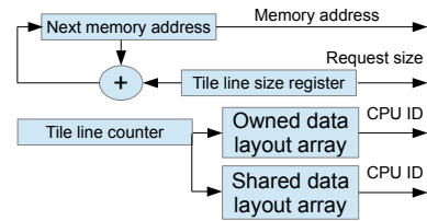
Figure 6: An outline of the memory access logic for data arrays with flexible mapping. Since accessing a tile line in the DRAM requires many cycles, these circuits are pipelined to avoid extending the CMS engine critical path.
